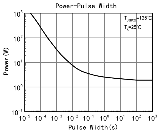
Figure 9: Single Pulse Power Rating Junction to Ambient
