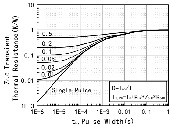
Figure 12. Transient Thermal Resistances
