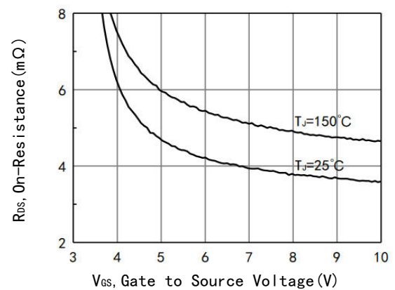
Figure 6. R_{DS(on)} vs. V_{GS}
