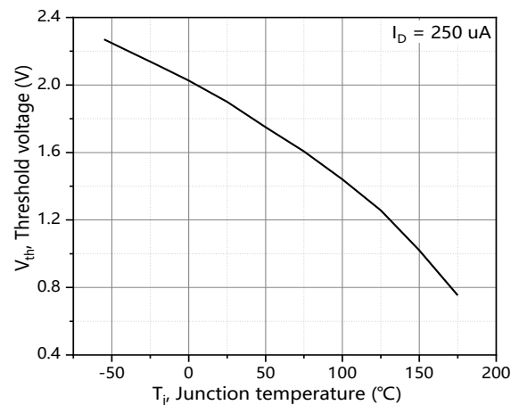
Figure 6. Threshold voltage
