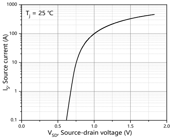
Figure 9. Diode Forward Characteristic
