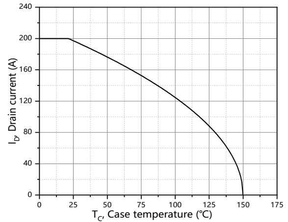
Figure 2. Drain current
