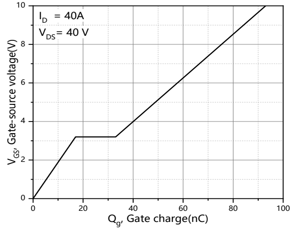
Figure 8. Gate Charge Characteristic
