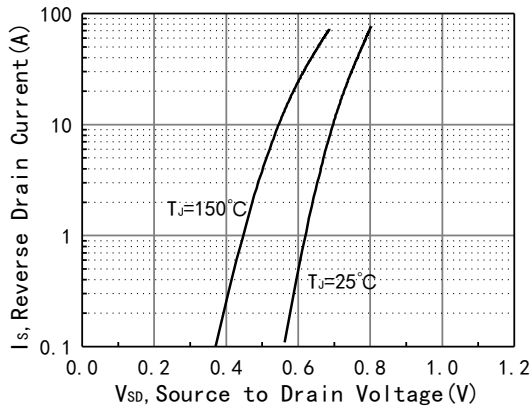
Figure 9. Diode Forward Characteristic
