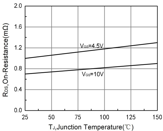
Figure 5. R_{DS(on)} vs. T_J
