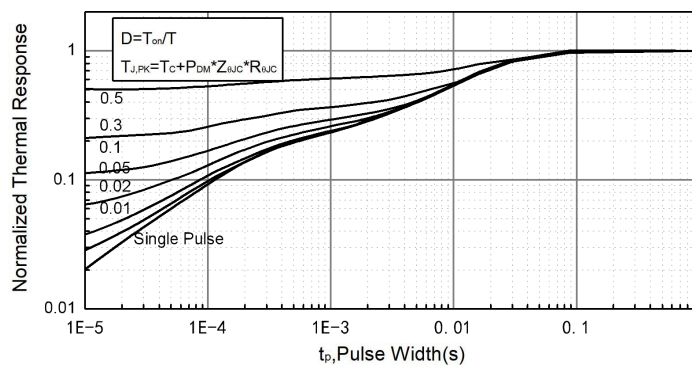
Figure 11. Normalized Maximum Transient Thermal Impedance
